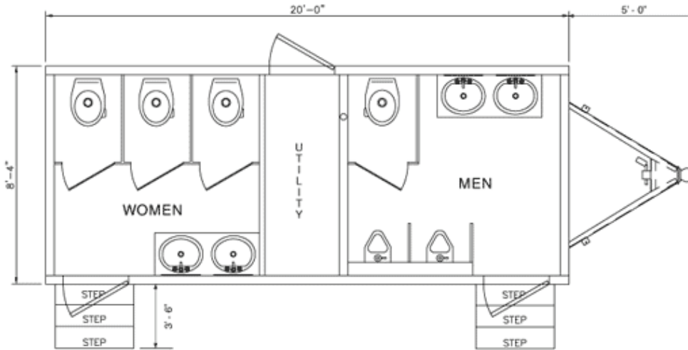
OVERALL LENGTH INCLUDING TONGUE AND HITCH: 25 FEET / OVERALL WIDTH WITH STEPS DEPLOYED: 11 FEET 10 INCHES
