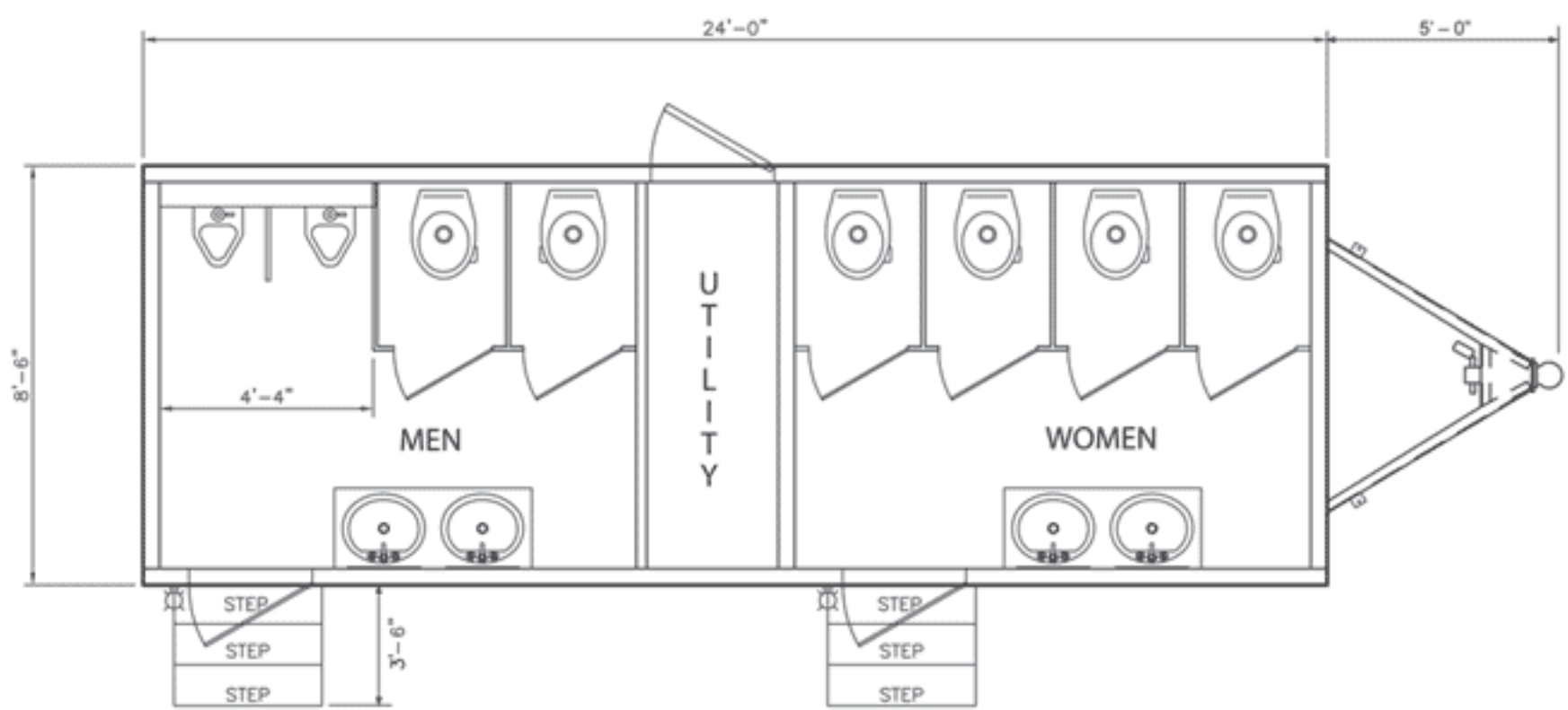
OVERALL LENGTH INCLUDING TONGUE AND HITCH: 29 FEET / OVERALL WIDTH WITH STEPS DEPLOYED: 12 FEET
